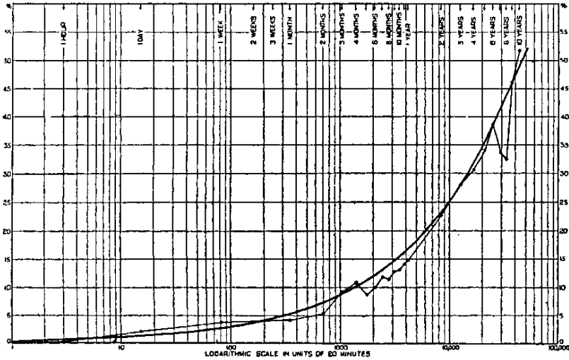
FIGURE 2.—Absolute percentage changes in stock price indexes.
